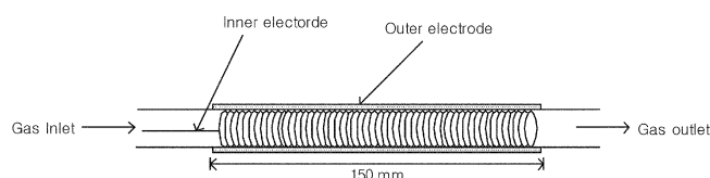
Fig. 2. Construction of the dielectric-barrier discharge reactor.
